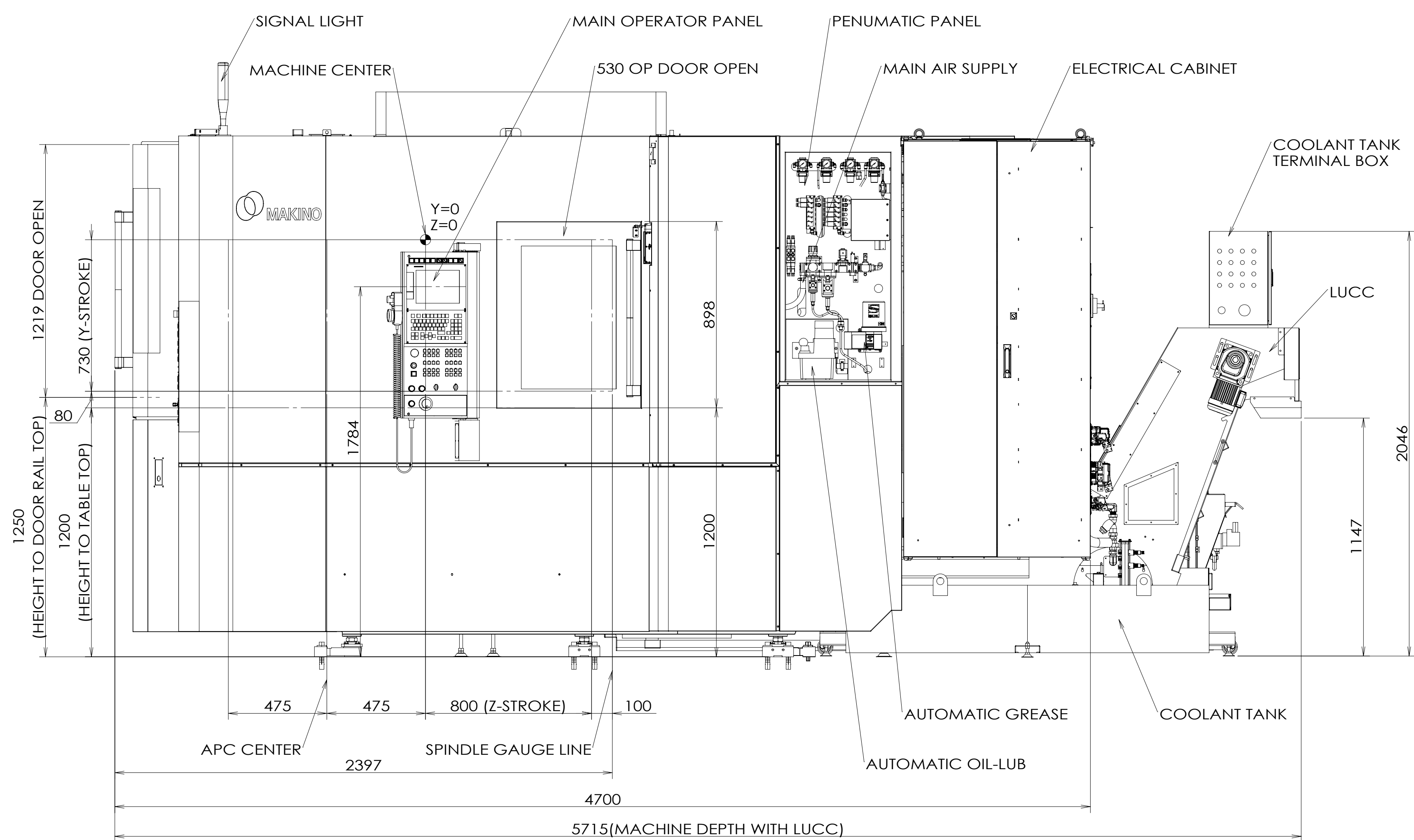
RIGHT SIDE VIEW
